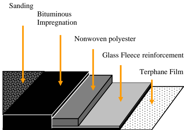
Figure 2: Typical cross-section
