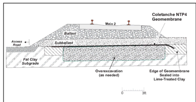
Figure 1: Design Cross Section
